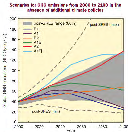
Figure 3.1. Global GHG emissions (in GtCO 2 -eq per year) in the absence of additional climate policies: six illustrative SRES marker scenarios (coloured lines) and 80 th percentile range of recent scenarios published since SRES (post-SRES) (gray shaded area). Dashed lines show the full range of post-SRES scenarios. The emissions include CO 2 , CH 4 , N 2 O and F-gases. {WGIII 1.3, 3.2, Figure SPM.4}
